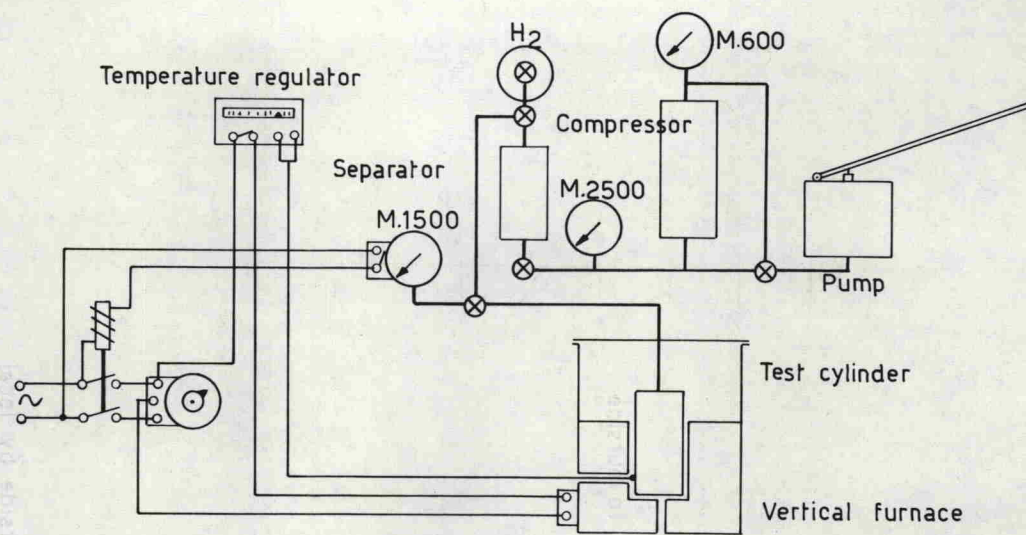
Experimental device
